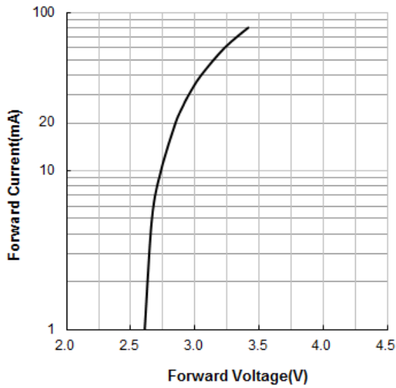
Forward Voltage vs. Forward Current (Ta=25°C)
